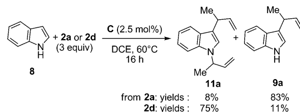
Scheme 4. Alkylation of 8 from linear and branched allyl alcohols. Yields shown are those of isolated products.
